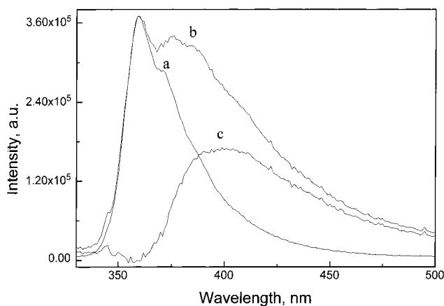
Figure 7. Fluorescence spectra of 5 in tetrahydrofuran (a) without DABCO, (b) with 5.5 mM DABCO, and (c) the difference of the normalized spectra (b – a).
